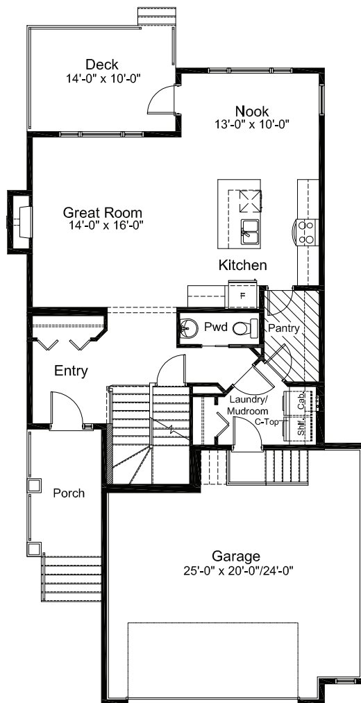
MAIN FLOOR 947 sq. ft.
