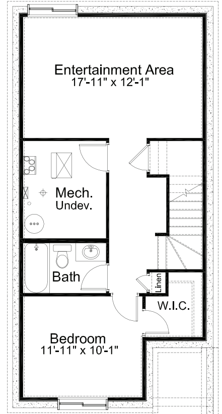
Basement Development Option 544 sq. ft. of developed area
