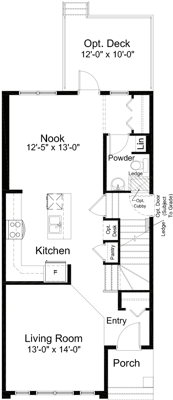
MAIN FLOOR 764 sq. ft.
