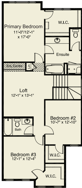
Primary Bedroom Extension & Central Loft Option w/ Added Linen & Entertainment Centre (must be combined with Main Floor Laundry Option) 1,193 sq. ft.
