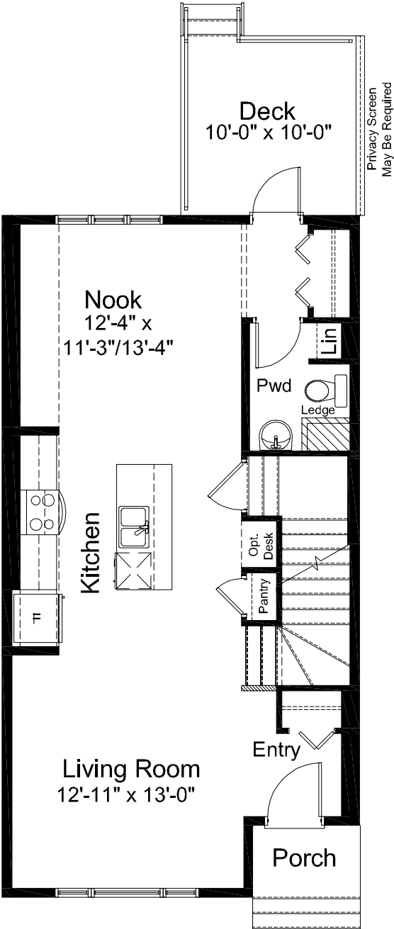
MAIN FLOOR 733 sq. ft.
