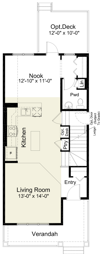
Kitchen Layout Option # 1
