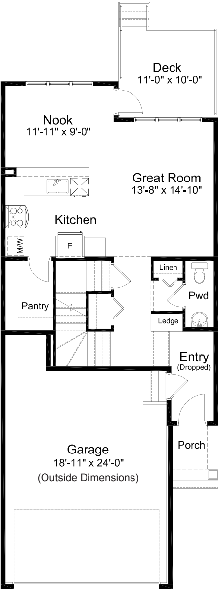
MAIN FLOOR 737 sq. ft.
