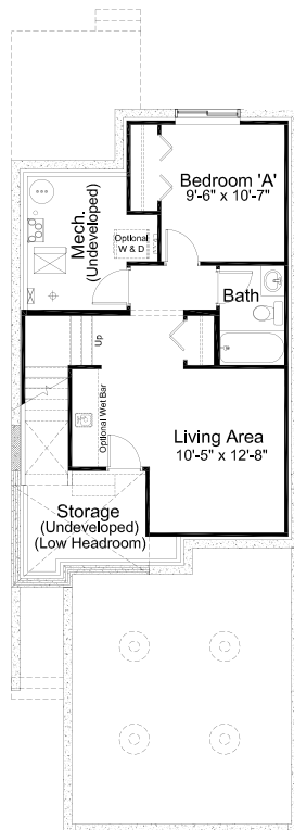
Basement Development for Side Entry Option 435 sq. ft. of developed area
