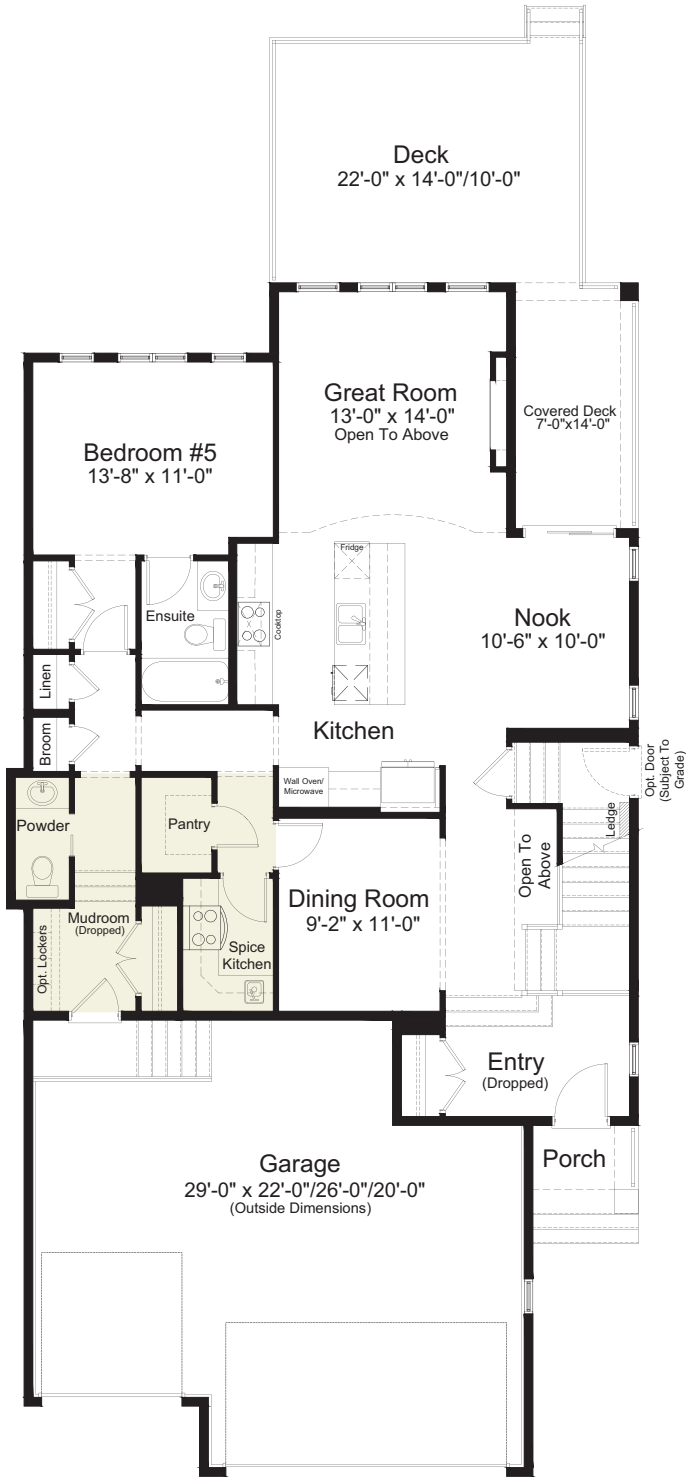
Spice Kitchen Option main floor: 1,408 sq. ft.
