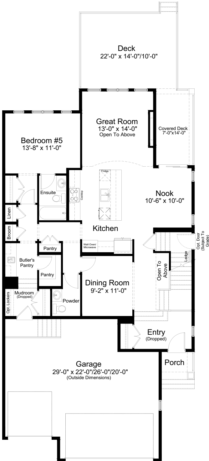
MAIN FLOOR 1,400 sq. ft.
