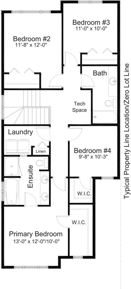
UPPER FLOOR 1,168 sq. ft.
