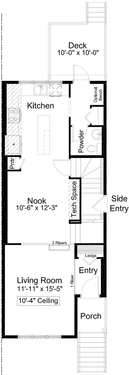
MAIN FLOOR 757 sq. ft.
