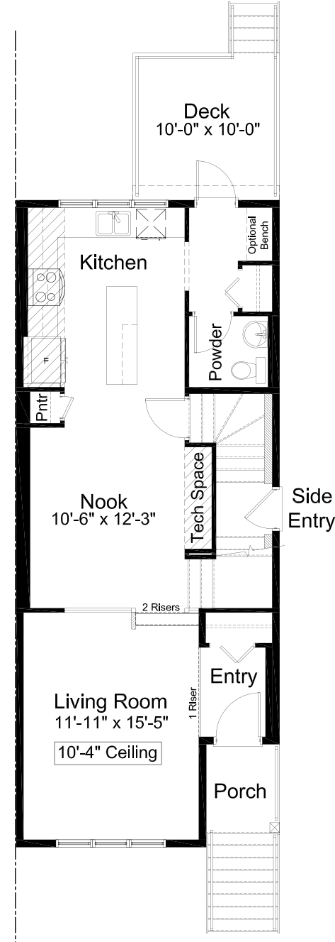
MAIN FLOOR 757 sq. ft.
