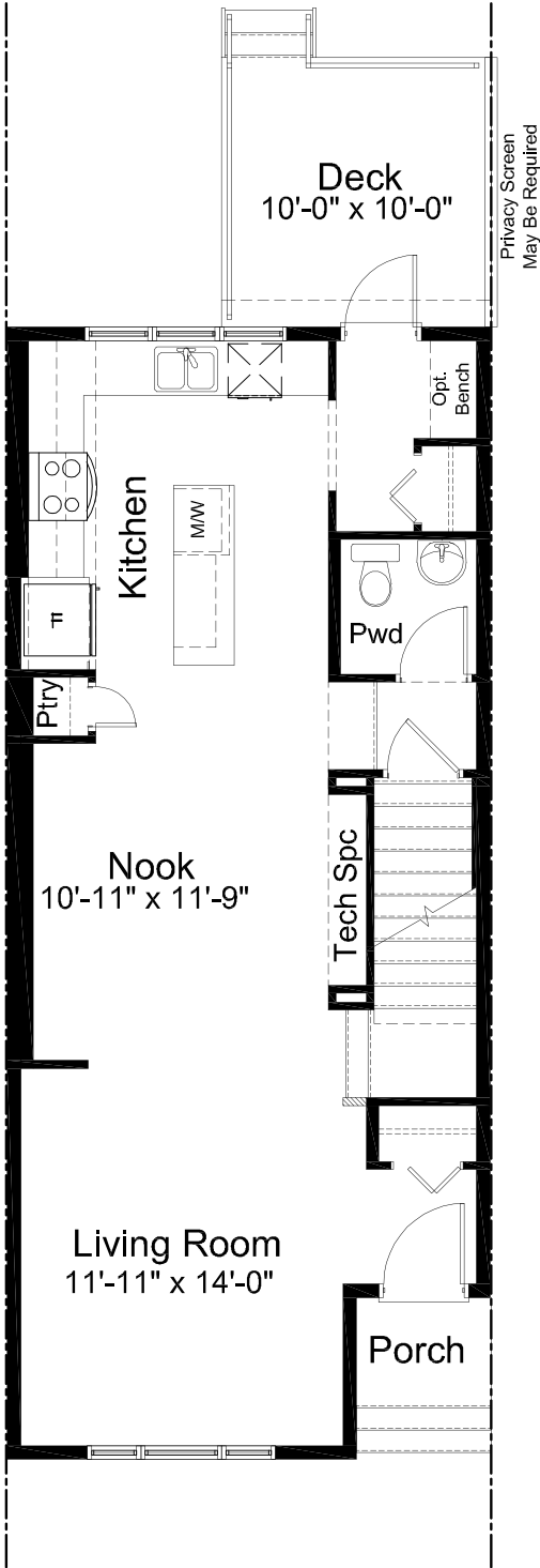
MAIN FLOOR 723 sq. ft.
