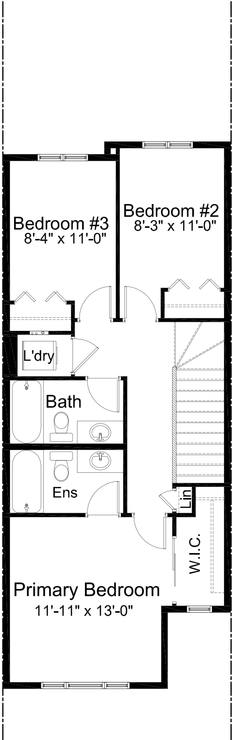
UPPER FLOOR 733 sq. ft.
