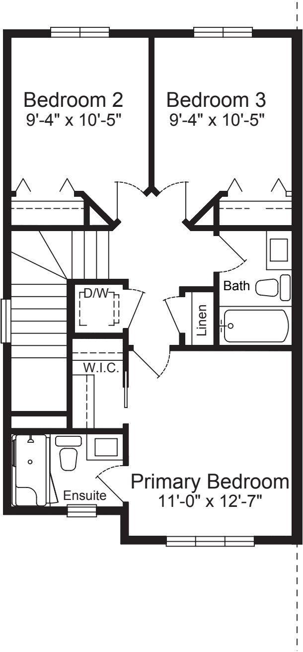
UPPER FLOOR 684 sq. ft.
