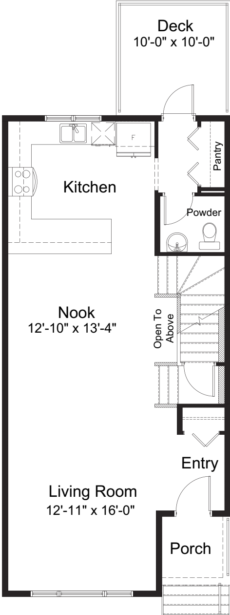
MAIN FLOOR 796 sq. ft.
