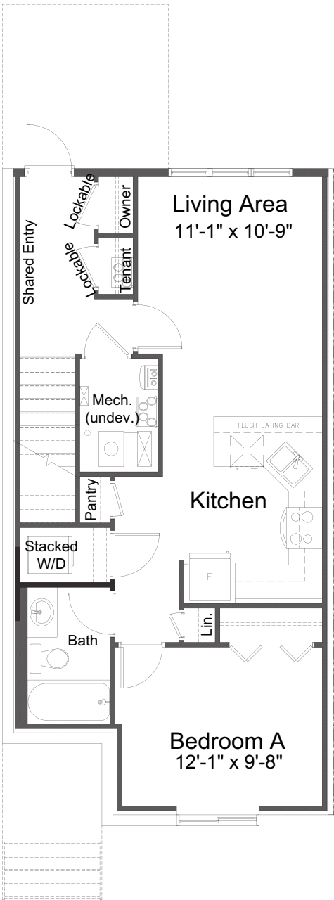
BASEMENT SUITE 647 sq. ft.
